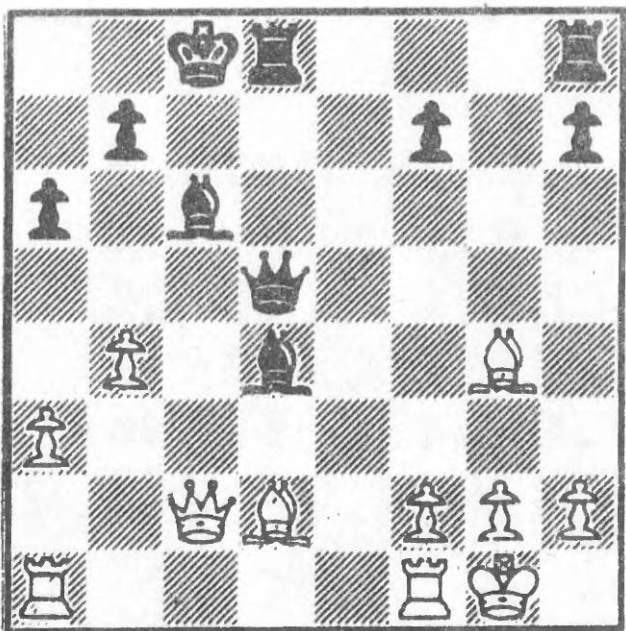
269 After 22 Bxg4+
